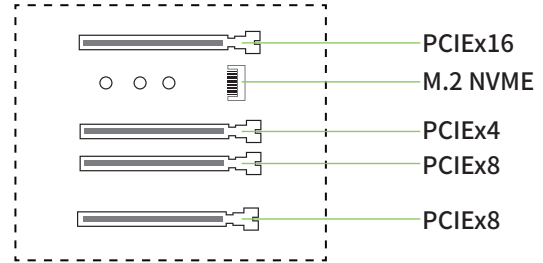
2-4 PCI Expansion Slot
